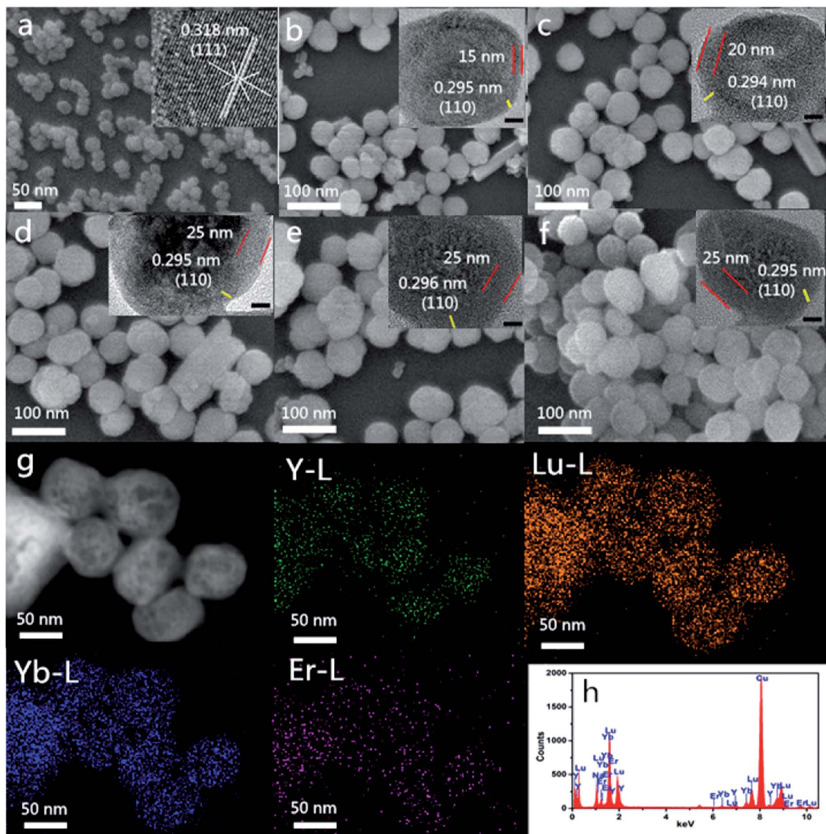
Fig. 2 SEM images of NaYF 4 :Yb/Er (a), NaYF 4 :Yb/Er@NaLuF 4 :Yb with reaction time of 2 h (b), 3 h (c), 4 h (d), UCNP-OAO (e), UCNP-PEI (f), respectively; elemental mapping and EDS of NaYF 4 :Yb/Er@NaLuF 4 :Yb with reaction time of 4 h (g) and (h), respectively. Insets in (a)–(f) show HR-TEM images of UCNP. Scale bars represent 20 nm for insets.
