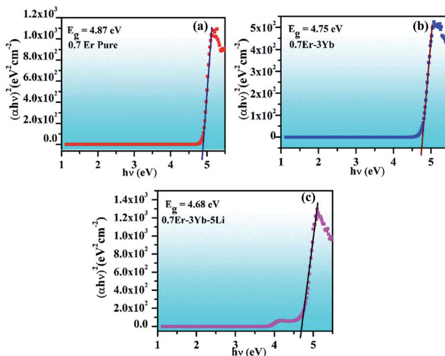
Fig. 6 Plots between (\alpha h\nu)^2 versus h\nu for the (a) 0.7\text{Er}^{3+} , (b) 0.7\text{Er}^{3+}/3\text{Yb}^{3+} , and (c) 0.7\text{Er}^{3+}/3\text{Yb}^{3+}/5\text{Li}^+ doped and co-doped \text{ZnGa}_2\text{O}_4 phosphors.
