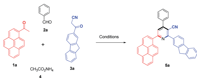
Scheme 1 Model reaction.
