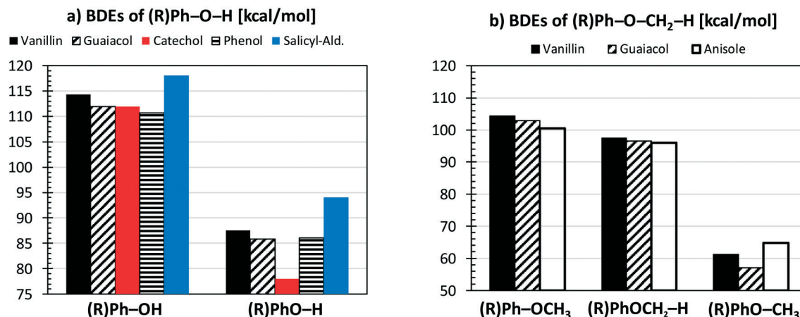
Fig. 4 Comparison of vanillin BDEs [ \text{kcal mol}^{-1} ] with respect to different aromatic compounds. Panel a) hydroxyl group; panel b) methoxy group.
