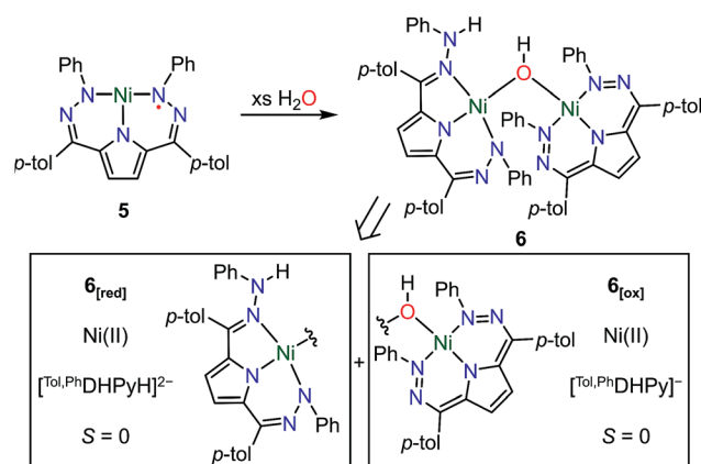
Scheme 2 Top: Synthesis of [Tol,PhDHPy]Ni(μ-OH)Ni[Tol,PhDHPyH] (6) and Bottom: Constituent oxidized (6 [ox] ) and reduced (6 [red] ) halves of the dimer.
