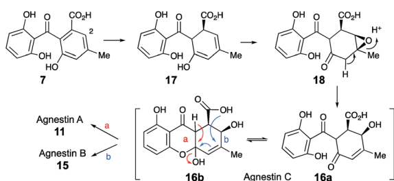
Scheme 2 Postulated formation of agnestins A 11 and B 15 via agnestin C 16ab .
