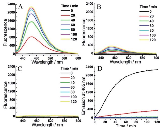
Fig. 2 Time-dependent fluorescent response of probe 1 ( 1 \mu\text{M} ) toward \text{H}_2\text{S} (200 \mu\text{M} ) and/or hNQO1 (1 \mu\text{g mL}^{-1} ). (A) 1 was treated with \text{H}_2\text{S} and hNQO1 simultaneously, or only with \text{H}_2\text{S} (B) or hNQO1 (C). (D) Time-dependent emissions at 465 nm for 1 treated with hNQO1 and \text{H}_2\text{S} (black), hNQO1 (green), \text{H}_2\text{S} (red) or probe 1 alone (blue) in PBS buffer.
