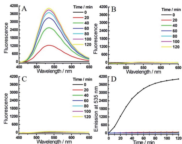
Fig. 3 Time-dependent fluorescent response of probe 2 ( 1 \mu\text{M} ) toward \text{H}_2\text{S} (200 \mu\text{M} ) and/or hNQO1 (1 \mu\text{g mL}^{-1} ). (A) 2 was treated with \text{H}_2\text{S} and hNQO1 simultaneously, or only with hNQO1 (B) or \text{H}_2\text{S} (C). (D) Time-dependent emissions at 535 nm for 2 treated with hNQO1 and \text{H}_2\text{S} (black), hNQO1 (green), \text{H}_2\text{S} (red) or probe 2 alone (blue) in PBS buffer.
