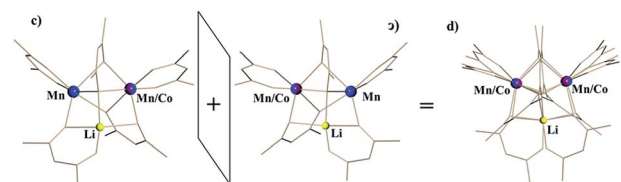
Fig. 5 Disordered unit (d) in the crystal structure of \text{LiMn}_{1.5}\text{Co}_{0.5}(\text{thd})_5 ( 1b ) as a superposition of two enantiomers ( S,A,A -c and R,A,A - \bar{c} ).
