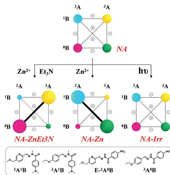
Scheme 4 Weighted graph representation of triple adaptation within the [2 \times 2] CDN NA from the statistical distribution (top) of the four constituents ^2\text{A}^1\text{B} , ^3\text{A}^1\text{B} , ^2\text{A}^8\text{B} and ^3\text{A}^8\text{B} (3.5 mM each) in response to 0.5 eq. \text{Zn}^{2+} & 1 eq. \text{Et}_3\text{N} (middle left), 0.5 eq. \text{Zn}^{2+} (middle center) and light irradiation ( \lambda_{\text{irr}} = 310\text{--}400\text{ nm} , middle right). † See text and ESI for conditions, catalyst and temperature. See Table S7† for numerical values.
