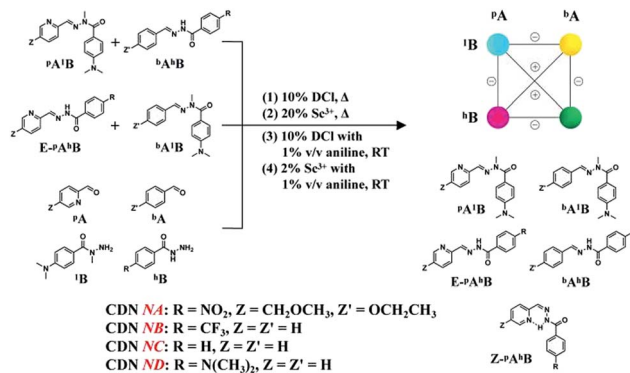
Scheme 1 Generation of four [2 \times 2] CDNs with four constituents ^p\text{A}^1\text{B} , ^p\text{A}^h\text{B} , ^b\text{A}^1\text{B} and ^b\text{A}^h\text{B} (3.5 mM each) by component exchange between either ^p\text{A}^1\text{B} and ^b\text{A}^h\text{B} (left top) or ^p\text{A}^h\text{B} and ^b\text{A}^1\text{B} (left middle), or by component condensation of ^p\text{A} , ^b\text{A} , ^1\text{B} and ^h\text{B} with different catalyst and temperature conditions, giving the same statistical distribution. ^p\text{A}^h\text{B} exist in both E and Z isomers. The diagonals and edges of the square link agonistic (+) and antagonistic (–) constituents, respectively.
