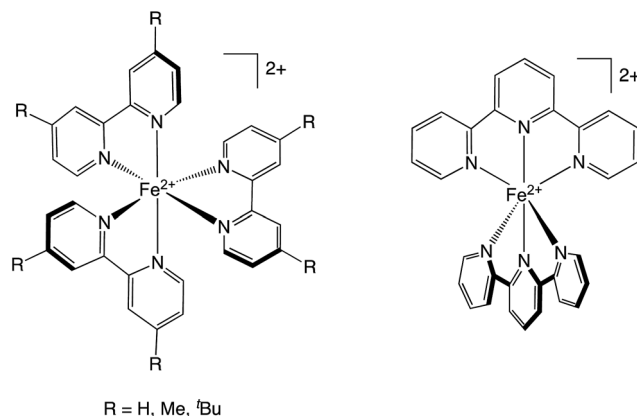
Chart 1 The four complexes used in these studies. Left: [\text{Fe}(\text{bpy}')_3]^{2+} family, in which R = H for [\text{Fe}(\text{bpy})_3]^{2+} , CH 3 for [\text{Fe}(\text{dmb})_3]^{2+} , and tert -butyl for [\text{Fe}(\text{dtbb})_3]^{2+} . Right: [\text{Fe}(\text{terpy})_2]^{2+} .
