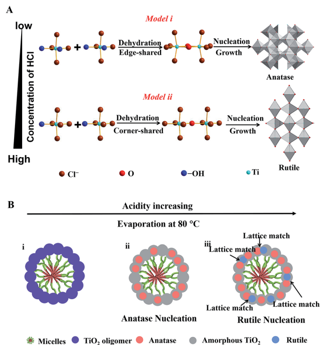
Scheme 1 (A) Schematic representation of the process of \text{TiO}_2 nucleation and cross-linking of [\text{Ti}(\text{OH})_n\text{Cl}_m]^{2-} octahedra during the solvent evaporation. There are two distinct cross-linking ways of [\text{Ti}(\text{OH})_n\text{Cl}_m]^{2-} octahedra under the different coordination conditions. (B) Schematic illustration of the nucleation and growth processes of \text{TiO}_2 nanocrystals during assembly with the amphiphilic triblock copolymer micelles via the coordination-mediated self-assembly method.
