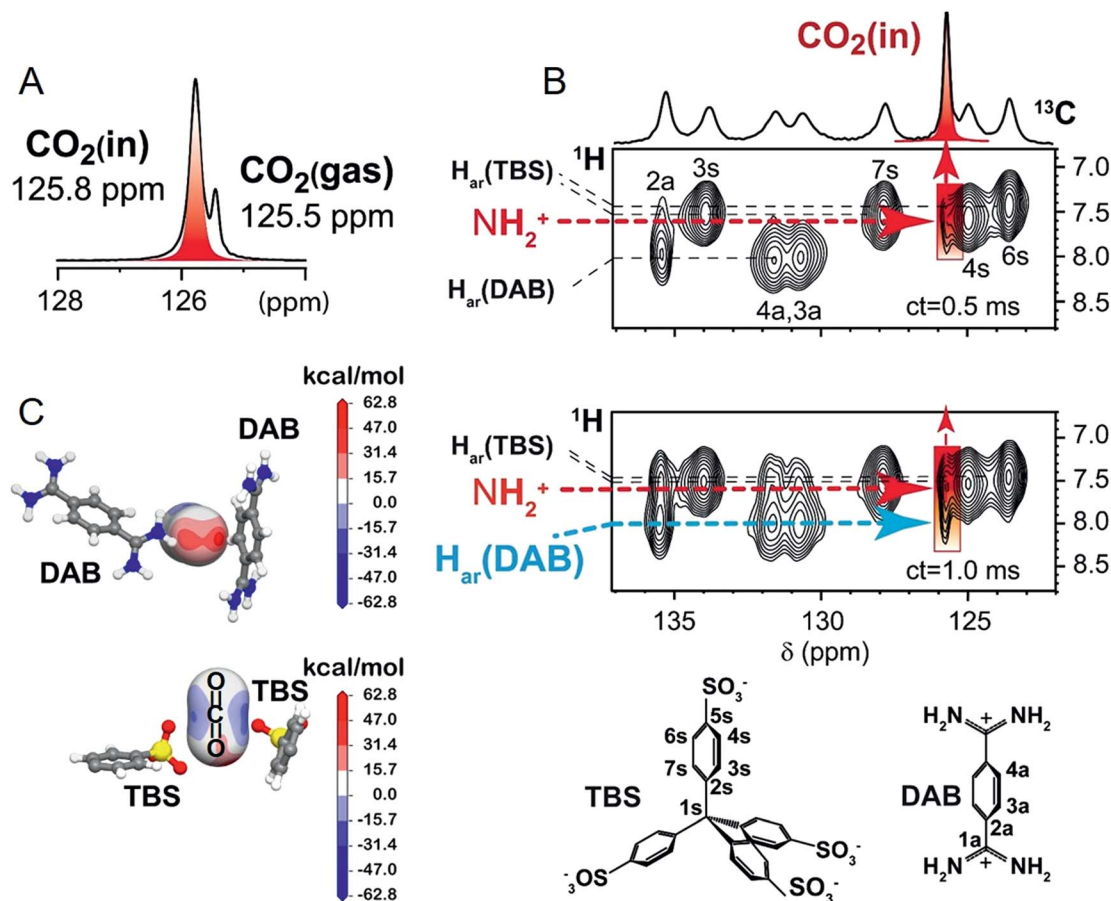
Fig. 3 CPOS-5 loaded with ^{13}\text{C} -enriched \text{CO}_2 (0.75 bar at RT): (A) ^{13}\text{C} MAS NMR spectrum; (B) 2D ^1\text{H}\text{--}^{13}\text{C} HETCOR MAS NMR spectra collected at room temperature and at two distinct contact times (ct). The host– \text{CO}_2 cross peaks are highlighted in red. Chemical structures of TBS and DAB with labels (below). (C) Electrostatic potential projected on \text{CO}_2 molecules by the DAB and TBS host moieties. The \text{CO}_2 molecules were localized by DFT calculations.
