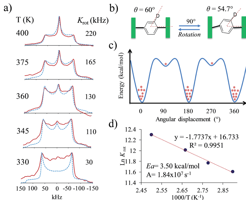
Fig. 6 (a) Comparison of the experimental and calculated 2 H line shapes, (b) distortion of the molecular axis, (c) representation of the asymmetric rotational potential and (d) Arrhenius plot with resulting activation parameters.
