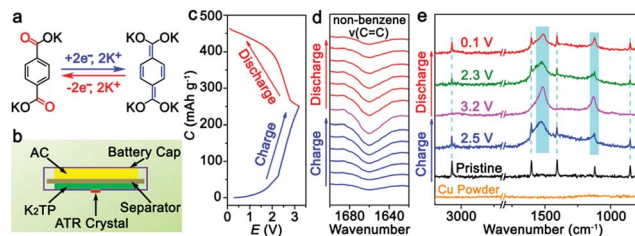
Fig. 2 (a) Redox reaction mechanism of K^+ with K_2TP ; (b) diagram of a cell for in situ FTIR test; (c) charge/discharge profile of the KHC at 20\text{ mA g}^{-1} (based on the mass of K_2TP ); (d) in situ FTIR spectra of the K_2TP negative electrode in a charge/discharge cycle; and (e) Raman spectra of the K_2TP negative electrode at selected states with copper powder.
