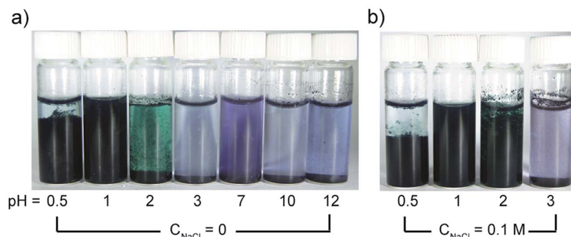
Fig. 7 (a) Optical images of TANI dispersed in aqueous solutions ( 2 \text{ mg mL}^{-1} ) at different pH and (b) with 0.1 \text{ M NaCl} added after standing for 15 hours.
