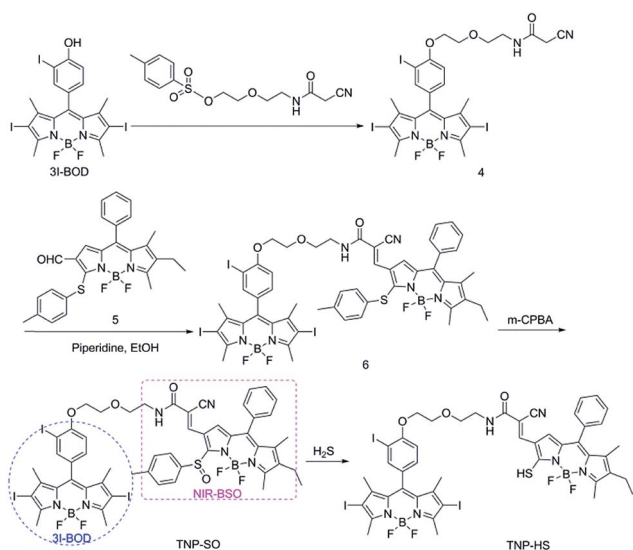
Scheme 1 Synthesis of the target compound TNP-SO.
