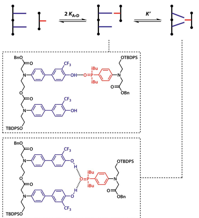
Fig. 8 Pathway towards formation of a double hydrogen bond between DD 2-mer and A. K_{A \cdot D} is the intermolecular association constant for formation of a single A · D hydrogen bond, K' is the association constant for the interaction of the second phenol with the same phosphine oxide. Statistical factors represent the degeneracy of the structures involved.
