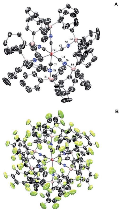
Fig. 1 (A) Molecular structure of (\text{TEA})_4[\text{Fe}(\text{CN}-\text{BPh}_3)_6] ( 2 ). Thermal ellipsoids set at 50% probability. Cations and protons omitted for clarity. Selected bond distances and angles: Fe1–C1: 1.908(7) Å, Fe1–C3: 1.913(8) Å, Fe1–C4: 1.908(8) Å, C1–N1: 1.170(9) Å, C3–N3: 1.164(10) Å, C4–N4: 1.166(10) Å, N1–B1: 1.559(9) Å, N3–B3: 1.573(10) Å, N4–B4: 1.557(10) Å, Fe1–C1–N1: 174.0(7)°, Fe1–C3–N3: 174.0(7)°, Fe4–C4–N4: 179.6(8)°, C1–N1–B1: 172.0(8)°, C3–N3–B3: 173.5(8)°, C4–N4–B4: 176.3(7)°. (B) Molecular structure of (\text{PPN})_4[\text{Fe}(\text{CN}-\text{B}(\text{C}_6\text{F}_5)_3)_6] ( 3 ). Thermal ellipsoids set at 50% probability. Cations omitted for clarity. Selected bond distances and angles (labels as in 2 ): Fe1–C1: 1.899(4) Å, Fe1–C3: 1.904(3) Å, Fe1–C4: 1.897(3) Å, C1–N1: 1.146(4) Å, C3–N3: 1.152(4) Å, C4–N4: 1.160(4) Å, N1–B1: 1.545(5) Å, N3–B3: 1.550(5) Å, N4–B4: 1.551(4) Å, Fe1–C1–N1: 176.9(3)°, Fe1–C3–N3: 177.9(3)°, Fe1–C4–N4: 175.9(3)°, C1–N1–B1: 173.2(3)°, C3–N3–B3: 175.1(3)°, C4–N4–B4: 173.3(4)°.
