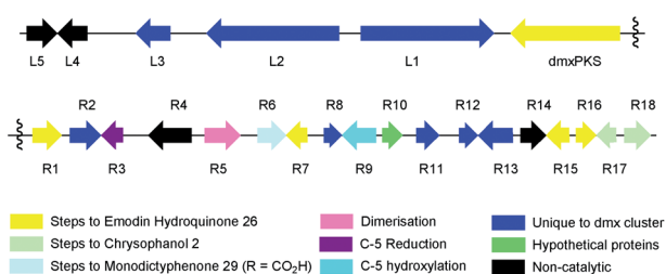
Fig. 5 Map of the cryptosporioptide dimeric xanthone ( dmx ) BGC coloured by proposed function (see Table 1). Not to scale.
