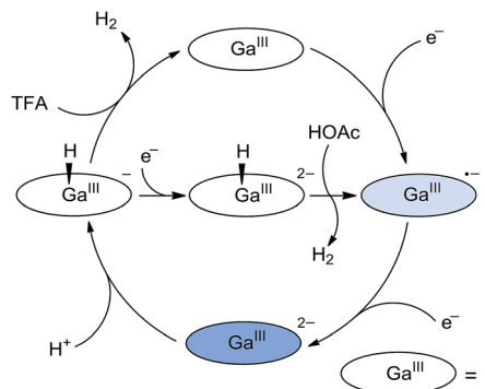
Fig. 5 Proposed catalytic cycles for the HER by 1 with the use of either TFA or acetic acid as the proton source.
