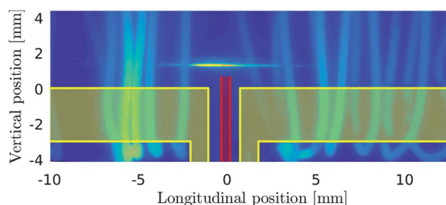
Fig. 3 Photographic image of the TALIF H fluorescence in the central lower section of the atomizer's optical arm. The image is supplemented with a schematically represented cross-section (i) of the appropriate part of the lower horizontal wall (thickness of 3 mm) of the optical arm (including the upper section of the inlet arm) highlighted in yellow and (ii) of the capillary walls highlighted in red.
