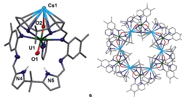
Fig. 6 Solid state structure of 9, depicting the asymmetric unit (left) and the hexanuclear Cs 1 –uranyl(v) ring (right). For clarity, all hydrogen atoms except pyrrole N–Hs and all solvent molecules are omitted (displacement ellipsoids are drawn at 50% probability). Selected bond distances (Å) and angles (°): U1–O1 1.857(6), U1–O2 1.833(6), O1–N4 3.01(1), O1–N5 2.92(1), O1–U1–O2: 175.2(3)°, Cs1–O2–U1 117.6(3)°; selected ring parameters (Å): Cs1–Cs1''' 13.4807(9), U1–U1''' 16.518(1); cavity size: 648 Å 3 .
