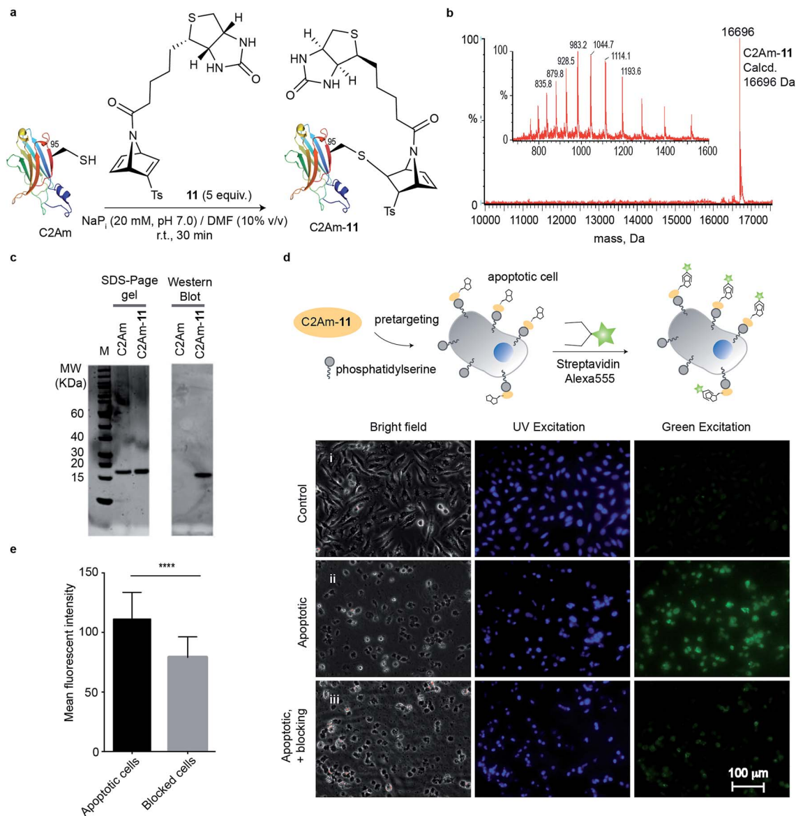
Fig. 3 Imaging of apoptotic HeLa cells with C2Am-11. (a) Reaction between C2Am and 11 in NaPi (20 mM, pH 7.0) at 25 °C for 30 min. (b) Deconvoluted mass spectrum obtained from a representative reaction. (c) Treatment of C2Am-11 with Streptavidin-Alexa555 after SDS-PAGE and membrane transfer gave a single fluorescent band as detected by Western blot that confirms biotinylation of C2Am and binding of the fluorescent streptavidin to the biotin. Lanes 1 and 2, Spyro Protein Ruby staining (SDS-PAGE); lanes 3 and 4, fluorescence at excitation and emission wavelengths for Alexa 555 (Western Blot membrane). (d) Epifluorescent images of non-apoptotic (control) and apoptotic HeLa cells after labelling with C2Am-11 + Streptavidin Alexa555. Blocking studies were performed by pre-incubating apoptotic cells with an excess of non-fluorescent C2Am before incubation with C2Am-11 + Streptavidin Alexa555. Apoptotic cells are shown in green. Blue represents Hoechst-stained nuclei. (e) MFI from apoptotic and blocked cells determined with ImageJ (average of 30 regions of interest). Statistical significance was determined by paired t test by using GraphPad Prism (****, P < 0.0001 ).
