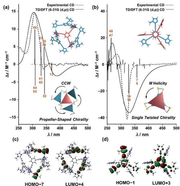
Fig. 8 Dashed lines show experimental CD spectra of (a) (\text{Im}^{\text{R/S}}_3\text{Bz})_4(\text{Zn}^{2+})_3 (corresponding to the red line in Fig. 4) and (b) (\text{ImH}_2)_m(\text{Im}^{\text{R/S}}_3\text{Bz})_2(\text{Zn}^{2+})_3 (corresponding to the yellow line in Fig. 5). Solid lines show theoretical CD spectra [TD-DFT/B3LYP-6-31G(d,p)] of the C_3 -symmetric ligands in (a) the propeller-shaped arrangement and (b) twisting dimer arrangement. Calculated spectrum in (a) is vertically scaled (scaling factor = 0.85). The numbered excitations correspond to those with high rotatory strength. Two molecular orbitals involved in (c) excitation 43 (17%) in (a) and (d) excitation 14 (47%) in (b). Insets: schematic representation of (a) propeller-shaped chirality and (b) single twisted chirality.
