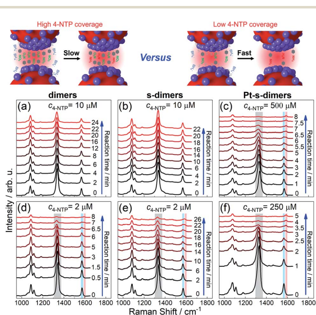
Fig. 4 SERS tracking of \text{NaBH}_4 -based hydrogenation of 4-NTP adsorbed on AuNP dimers (a and d), s -dimers (b and e), and Pt- s -dimers (c and f) with 4-NTP incubation concentrations indicated on each panel. See Fig. S25† for kinetic SERS data of Pd- s -dimers.
