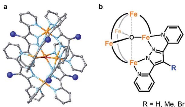
Scheme 2 Schematic illustrations of the series of pentanuclear iron complexes bearing 4-substituted-3,5-bis(pyridyl)pyrazole (R-Hbpp ( \text{R} = \text{H, Me, and Br} )) ligands investigated in this study.
