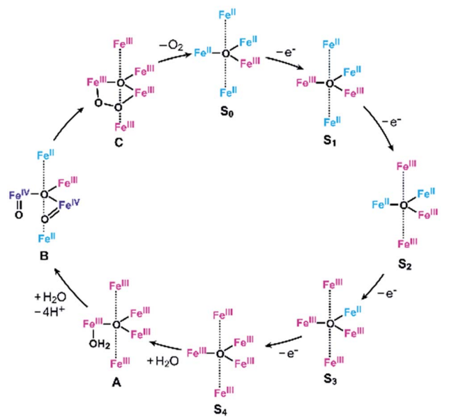
Fig. 5 Proposed reaction mechanism for the water oxidation catalyzed by [Fe 5 -Me] 3+ and [Fe 5 -H] 3+ . 33 Fe II , blue; Fe III , red; and Fe IV , purple.
