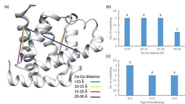
Fig. 6 Assessment of cross linkages with the myoglobin 3D structure: (a) cross-links mapped onto the crystal structures of myoglobin (PDB entry 1dwr); (b) distribution of the \text{C}\alpha\text{-C}\alpha distance of the identified linkages; and (c) types of cross-linking sites identified from the pBVS cross-linked myoglobin sample, with numbers indicated on top.
