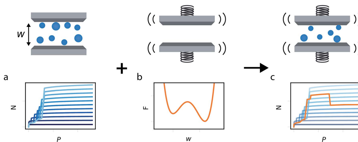
Fig. 1 Illustration of the methodology used to chart representative gas adsorption isotherms of responsive porous materials. (a) A series of isotherms at different pore widths, identified by different shades of blue. (b) The free energy profile describing the pore width. (c) A responsive isotherm calculated from the series of isotherms, as the minimum of \Omega_{os} , and identified by an orange path.
