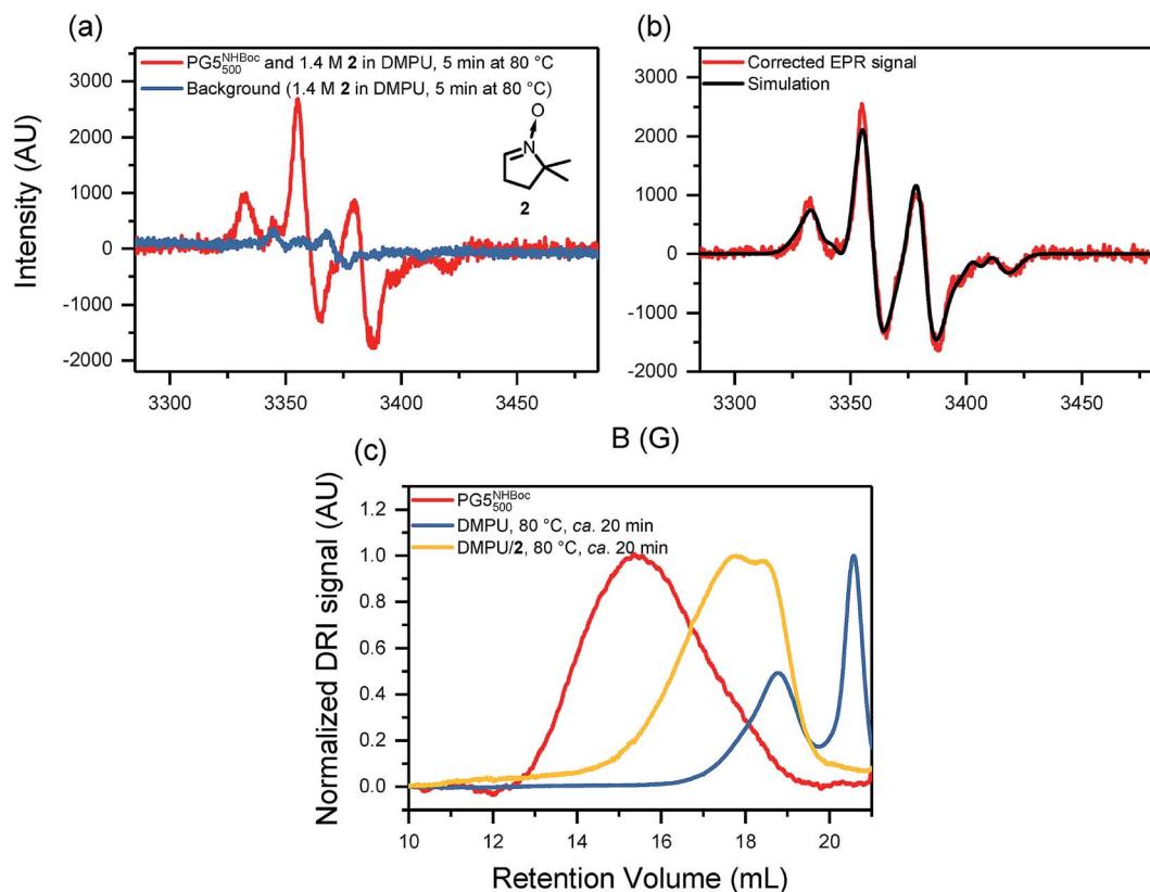
Fig. 8 (a) EPR spectra (200 K, X-band, 1 scan) after "hot solvent" treatment of \text{PG}_{500}^{\text{NH}^{\text{Boc}}} (ca. 5% w/v in 1.4 M DMPO/DMPU, 80 °C for 5 min). The inset shows the structure of the radical trapping agent DMPO (2). (b) Deconvolution of the background- and baseline-corrected EPR signal, consisting of 4 component radicals, see Fig. S41.† (c) GPC retention curves (DMF, 0.1% LiBr) of DPs isolated from EPR experiments after heating without and with a radical scavenger. Both samples were kept at 80 °C in DMPU for approx. 20 min.
