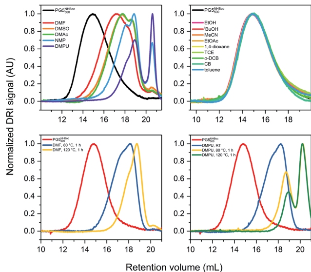
Fig. 3 GPC retention curves demonstrating the effects of solvent and temperature. Solutions of \text{PG}_{500}^{\text{NHBoc}} (1% w/v) were prepared at RT, then heated to the indicated temperature for 1 h. (a) Results obtained for polar-aprotic solvents in which scission was found to occur at 80 °C; (b) results obtained for other solvent categories (alcohols, intermediate polarity aprotic solvents, chlorinated solvents, aromatics) in which no scission was observed for T \leq 80 °C. Further heating of already degraded samples in (c) DMF and (d) DMPU up to 120 °C.
