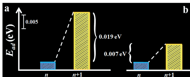
Fig. 4 Plots of the calculated sub-monolayer (a) and monolayer (b) adsorption energy of hexane, E_{\text{ad}} , on alkanethiolate monolayers ( n = odd).
