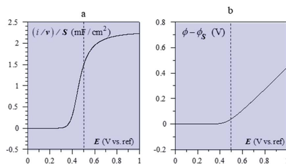
Fig. 9 (a) Forward CV scan for with C_d = 2.55 \text{ mF cm}^{-2} ( i.e. capacitance of a 40 nm CoP i film), F^2N/RT = 20 \text{ mF cm}^{-2} ( i.e. N = 8 \times 10^{20} \text{ cm}^{-3} for a 40 nm film), E^{0,\text{ap}} - \Delta E^0/2 + \phi_S = 0.5 \text{ V} (dashed vertical line), T = 298 \text{ K} . (b) Evolution of the film inner potential. Adapted from Fig. 5 in ref. 19 with permission.
