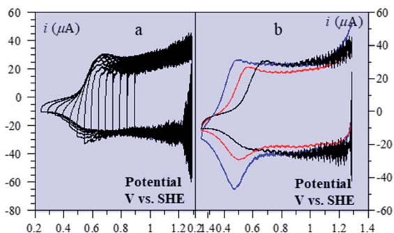
Fig. 7 (a) CV of a 39 nm CoP i film in 1 mM KP i , pH = 7, and 100 mM KNO 3 . Scans are initiated at 1.29 V vs. SHE in the cathodic direction and inversion potential is varying. \nu = 2 \text{ V s}^{-1} . (b) CV of a 39 nm CoP i film in the presence of 100 mM KNO 3 and 1 mM KP i , pH 7. Scans are initiated at 1.29 V vs. SHE in the cathodic direction. \nu = 2 \text{ V s}^{-1} . Films were deposited from different buffers: 100 mM KP i , pH 7 (black), 100 mM KHCO 3 , pH 10.3 (red), 100 mM KB i , pH 9.2 (dots).
