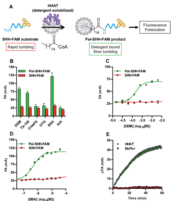
Fig. 1 Acyl-cLIP measurement of palmitoylation of a SHH N-terminus peptide. (A) Schematic representation of the Acyl-cLIP assay for HHAT. (B) Polarisation of substrate and product SHH-FAM peptides at 1 \mu M and detergents at 2 mM or BSA at 0.15 mM; only BSA and detergents above their CMC increase polarised emission of the lipidated peptide. (C) DDM titration demonstrates specific Pal-SHH-FAM polarised emission above the CMC. (D) BSA titration demonstrates specific Pal-SHH-FAM polarised emission above K_d . (E) Real-time analysis of SHH-FAM palmitoylation showing HHAT-dependent increase in FA over time. Data represent mean \pm SEM (assays performed in duplicate, n = 3 ).
