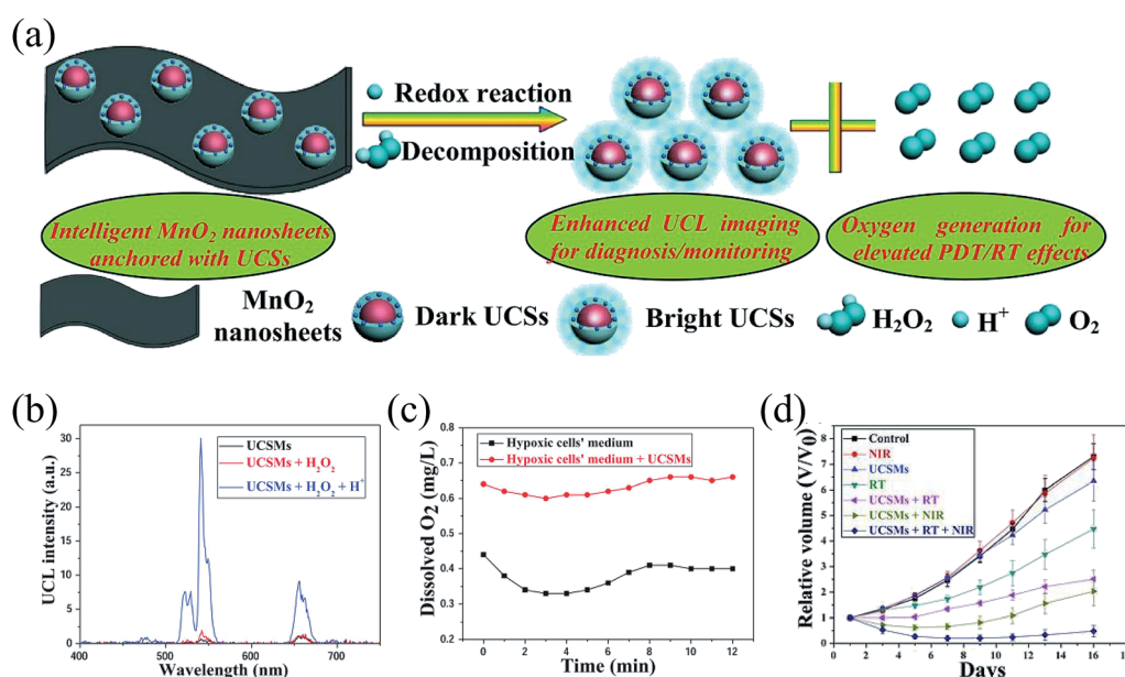
Fig. 3 MnO_2 nanosheets anchored by upconversion nanoparticles for oxygen-elevated synergetic therapy. 37 (a) Scheme of the decomposition of MnO_2 nanosheets from UCSMs attributed to the redox reaction between MnO_2 nanosheets and acidic H_2O_2 , resulting in the recovery of the upconversion luminescence and massive oxygen generation for enhanced PDT/RT. (b) Upconversion luminescence intensity for UCSMs under different conditions. (c) O_2 generation in hypoxic 4T1 cells treated with UCSMs. (d) Relative tumor growth curve of different groups of mice with different treatments. Adapted with permission from ref. 37. Copyright 2015 WILEY-VCH Verlag GmbH & Co. KGaA, Weinheim.
