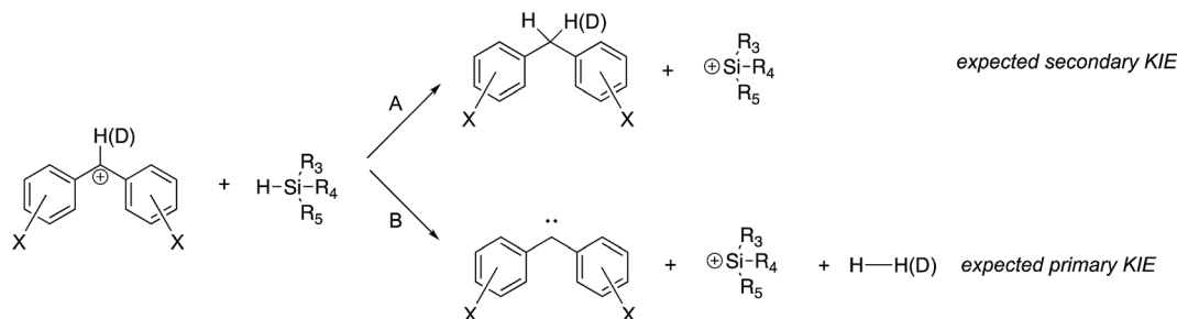
Fig. 4 Hydride abstraction versus proton abstraction.
