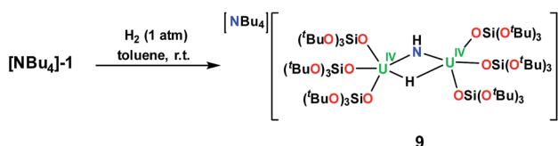
Scheme 6 Reaction of [\text{NBu}_4][\{(\text{LO})_3\text{U}\}_2(\mu\text{-NH})(\mu\text{-H})] with \text{H}_2 , 9 .
