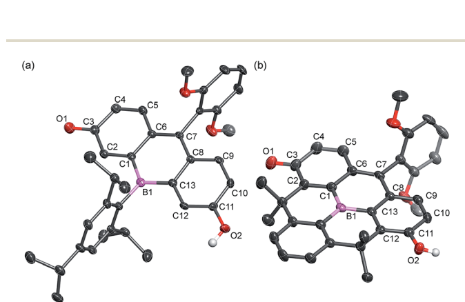
Fig. 2 Crystal structures of (a) BF2 and (b) BF3 (50% probability of thermal ellipsoids). Hydrogen atoms, except for those on the phenolic hydroxy groups, are omitted for clarity.
