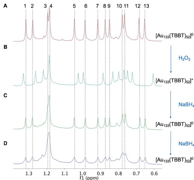
Fig. 5 Redox property of [\text{Au}_{133}(\text{TBBT})_{52}]^0 probed by NMR. (A) NMR of tert -butyl-H in [\text{Au}_{133}(\text{TBBT})_{52}]^0 . (B) Oxidation of [\text{Au}_{133}(\text{TBBT})_{52}]^0 to [\text{Au}_{133}(\text{TBBT})_{52}]^+ by \text{H}_2\text{O}_2 . (C) Reduction of [\text{Au}_{133}(\text{TBBT})_{52}]^+ to [\text{Au}_{133}(\text{TBBT})_{52}]^0 by \text{NaBH}_4 . (D) Further reaction of [\text{Au}_{133}(\text{TBBT})_{52}]^0 with \text{NaBH}_4 .
