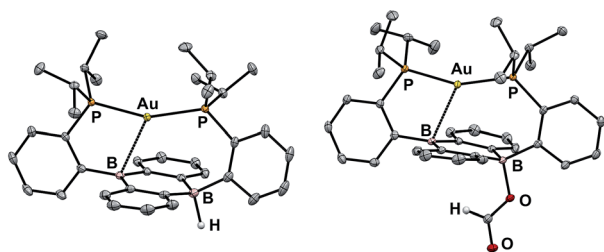
Fig. 3 Thermal ellipsoid plots (50%) of \text{Au}(\text{B}_2\text{P}_2)\text{H} (2, left) and \text{Au}(\text{B}_2\text{P}_2)(\text{O}_2\text{CH}) (5, right). Unlabeled ellipsoids correspond to carbon. Solvent molecules and most hydrogen atoms have been omitted for clarity.
