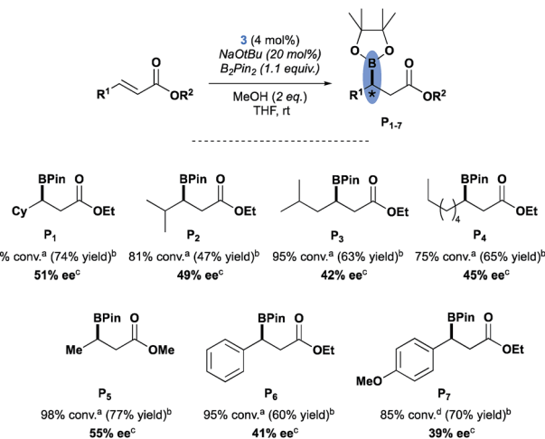
Scheme 7 Evaluation of Cholest CAAC CuCl complex 3 in ACB reaction. a Determined by 1 H NMR spectroscopy using mesitylene as an internal standard. b Isolated yield after SiO 2 purification. c Determined by GC on a chiral stationary phase (see ESI for details † ). d Anthracene was used as internal standard.
