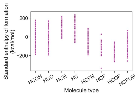
Fig. 4 Standard enthalpy of formation from G4MP2 calculations of the 133 K organic molecules classified into various groups of atom types.
