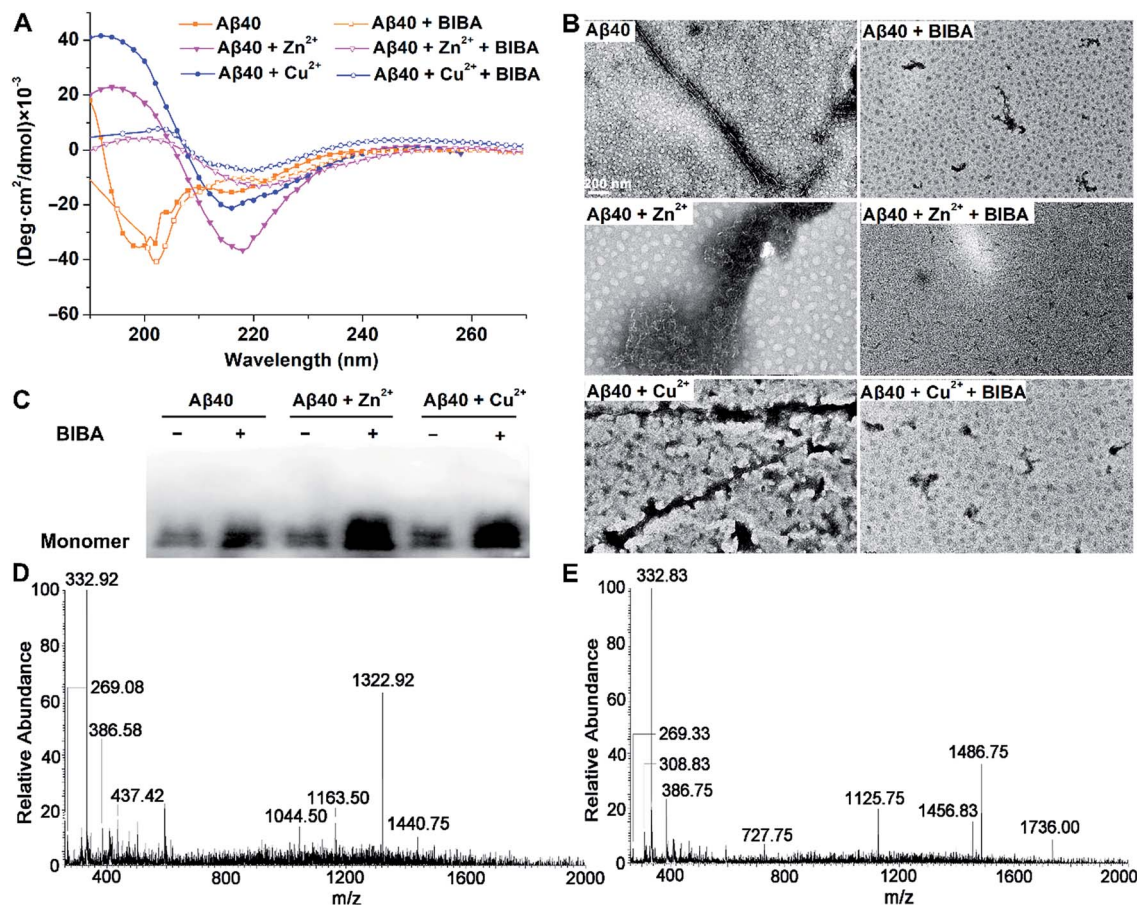
Fig. 2 Prevention of self- or metal-induced Aβ 40 aggregation by BIBA. (A) CD spectra, (B) TEM, and (C) Western blot of Aβ 40 without or with metal ions and BIBA, and ESI-MS spectra of Aβ 40 with (D) Zn 2+ or (E) Cu 2+ in the presence of BIBA ([Aβ] = [Zn 2+ /Cu 2+ ] = 10 μM and [BIBA] = 20 μM).
