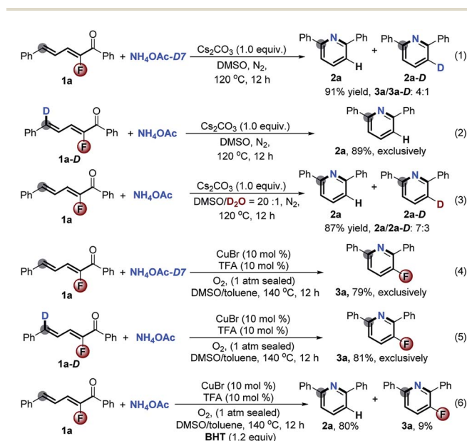
Scheme 6 Controlled reactions for mechanism investigation.
