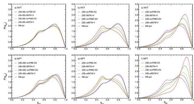
Fig. 4 Comparison between normalized probability distributions of the tetrahedral order parameter, P(q_{\text{tet}}) , calculated from PIMD simulations carried out at 298.15 K in the NVT (panels a–c) and NPT (panels d–f) ensembles with the (2B+3B)-XC PEFs (panels a and d), (2B)-XC PEFs (panels b and e), and (3B)-XC PEFs (panels c and f) with XC = revPBE-D3 (red), B97M-rV (yellow), revPBE0-D3 (green), and \omega B97M-V (magenta). Also shown in each panel are the corresponding distributions calculated from PIMD simulations with MB-pol.
