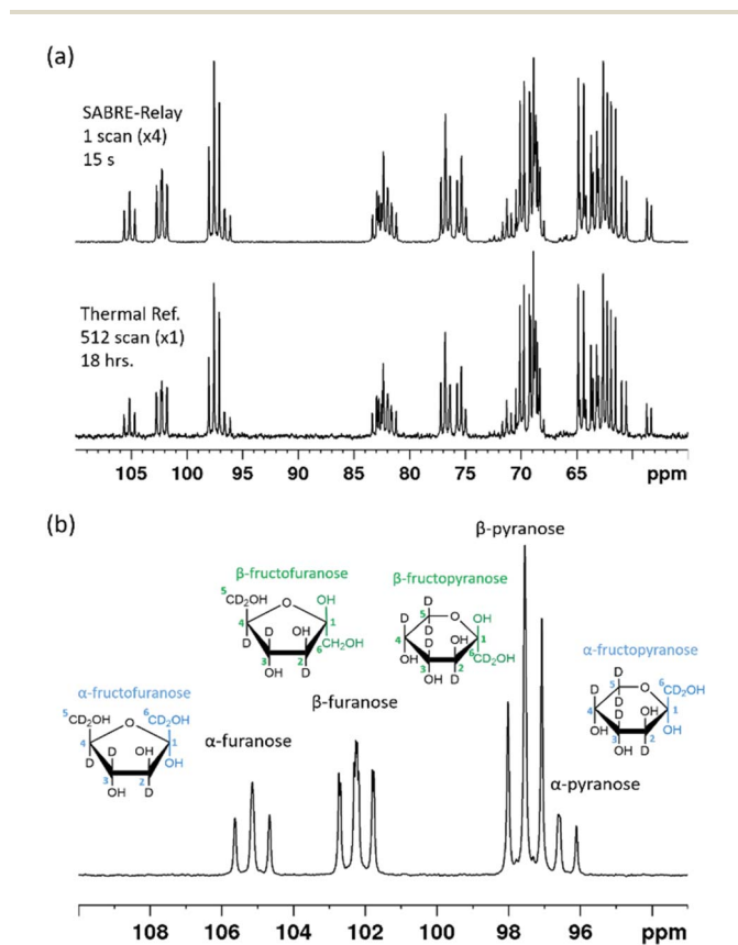
Fig. 8 (a) SABRE-Relay hyperpolarized ^{13}\text{C}\{^2\text{H}\} NMR spectrum of 19.9 mM of ^{13}\text{C}_6 - d_7 -fructose with 23.8 mM benzyl- d_7 -amine and 4.8 mM [\text{IrCl}(\text{COD})(\text{IMes})] of d_{22} -5 in a 0.65 ml \text{DCM-}d_2 : DMF (1.6 : 1) mixture measured at 9.4 T (top spectrum) with the corresponding thermal reference, averaged over 512 scans (bottom spectrum, 18 h). (b) Expansion of (a) to highlight the different isomeric forms indicated by their C-2 resonances.
