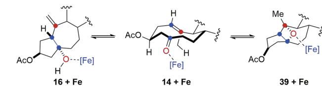
Fig. 3 (A) Computed energies comparing carbonyl-ene and oxetane-forming pathways. (B) Carbonyl-ene reaction and oxetane formation proceed reversibly under \text{FeCl}_3 -catalysis in transannular carbonyl-olefin metathesis.
