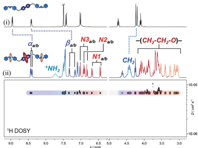
Fig. 2 ^1\text{H} NMR spectra (400 MHz, \text{CD}_3\text{CN} ) of (i) compound [\mathbf{1}\cdot\text{H}_2][\text{PF}_6]_4 and (ii) hetero[4]rotaxane \mathbf{p}\text{-H}[4]\mathbf{R} . ^1\text{H} DOSY NMR spectrum is shown in the bottom portion.
