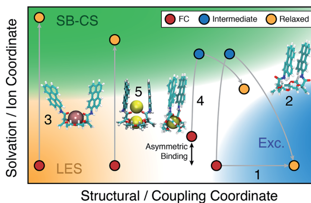
Fig. 9 Schematic two-dimensional representation of the relaxation pathways (gray lines) on the S_1 surface of the 18C6 host, 1 : 1 and 1 : 2 complexes (see text for details). FC: initial location at the ground-state geometry; LES: locally excited state; Exc.: excimer. The coloured area refer to the nature of the excited state.
