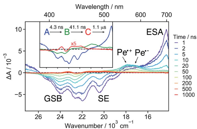
Fig. 6 Transient absorption spectra measured with 18C6 \subset Ba 2+ in acetonitrile at different time delays after 355 nm excitation. The evolution associated difference spectra (EADS) obtained from a global analysis assuming a sequential model are shown in the inset.
