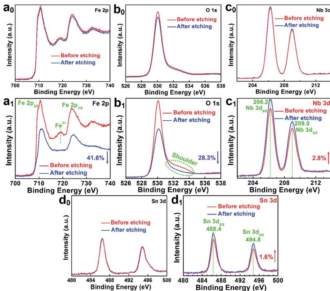
Fig. 3 XPS spectra of the pristine and activated Nb 2 Sn 2 Fe 2 O 3 photoanode before and after surface etching (~5 nm), respectively. (a 0 and a 1 ) Fe 2p. (b 0 and b 1 ) O 1s. (c 0 and c 1 ) Nb 3d. (d 0 and d 1 ) Sn 3d.
