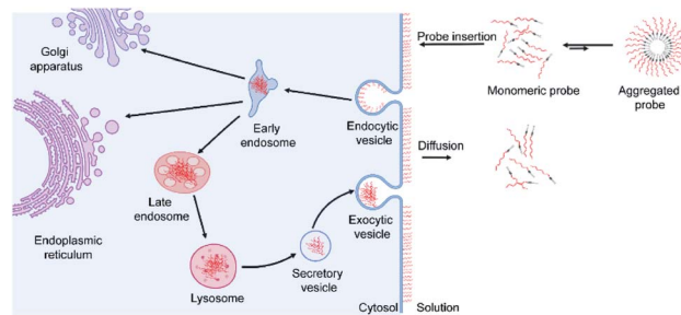
Fig. 6 Schematic of the dynamic process of lipid-DNA probe modification on cell membranes. First, there is equilibrium between the monomeric and aggregated forms of lipid-DNA probes in the solution. Monomeric form lipid-DNA probes insert into the cell membranes. Then, some of the cell membrane-anchored probes are internalized into the cells through the endocytosis pathway. Some membrane-anchored probes can also directly diffuse out into the extracellular solution or neighbouring cell membranes.
