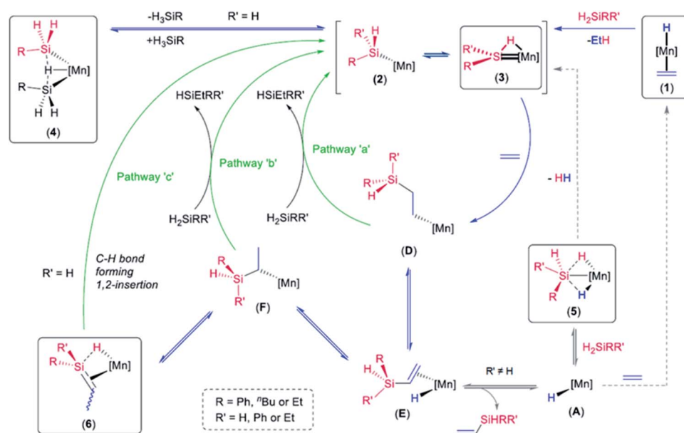
Scheme 8 Proposed catalytic cycle for ethylene hydrosilylation by primary and secondary hydrosilanes. [\text{Mn}] = \text{Mn}(\text{dmpe})_2 . Only one isomer is shown for complexes 3 and 5. Boxes represent complexes observed by NMR spectroscopy during catalysis.
